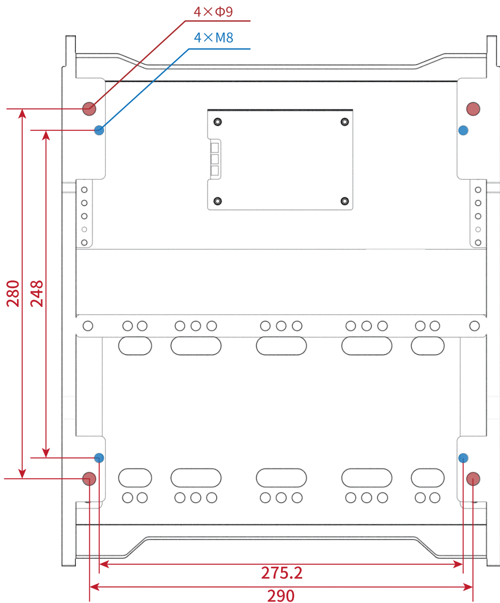
CPP EVO Drilling Template
