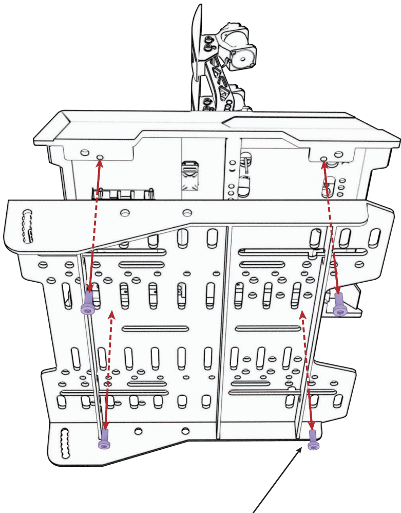
M8*16mm hex bolts (4 pieces)
